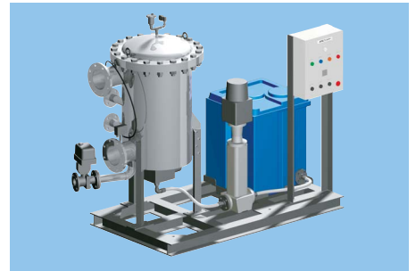
Auto reverse self-cleaning filter ARS Filter
