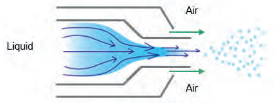
External mixing spray nozzles
