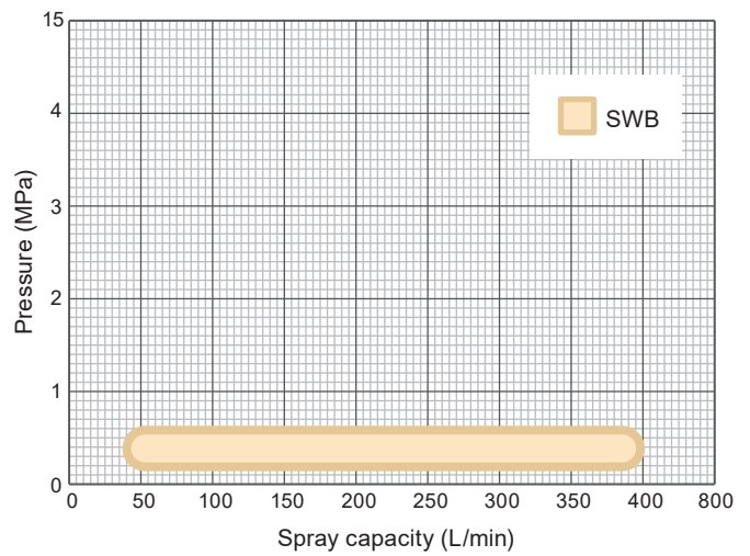
SWB Series
