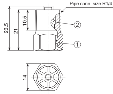
① Nozzle body ② Whirler
